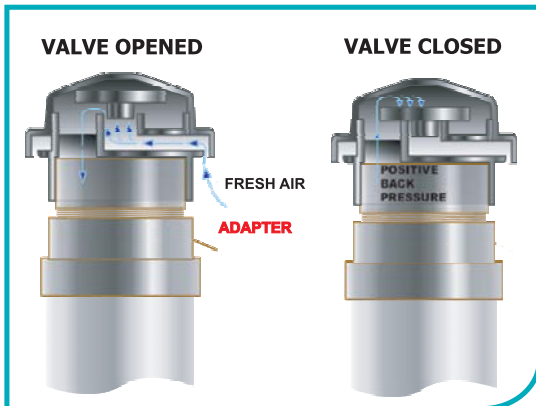
VP50 2" - 1 1/2" PVC AAV
